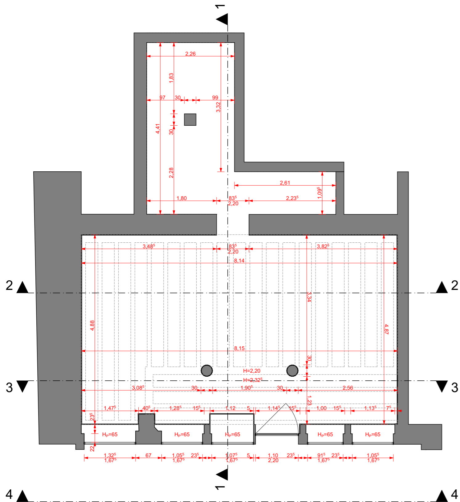
PLAN
